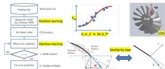
Machine learning of low-pressure fan noise
